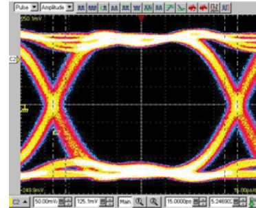
UJ-105RF with Fixture Rise Time: \approx 30 ps, Bit Rate: 8.75Gb/s PRBS ( Pseudo Random Bit Sequence ): 2^{10}-1
