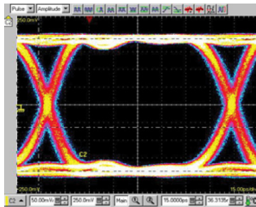
Through Fixture Rise Time: \approx 30 ps, Bit Rate: 8.75Gb/s PRBS ( Pseudo Random Bit Sequence ): 2^{10}-1
