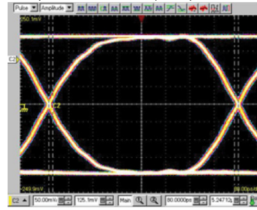
UJ-105RF with Fixture Rise Time: \approx 250 ps, Bit Rate: 1.6Gb/s PRBS ( Pseudo Random Bit Sequence ): 2^{10}-1
